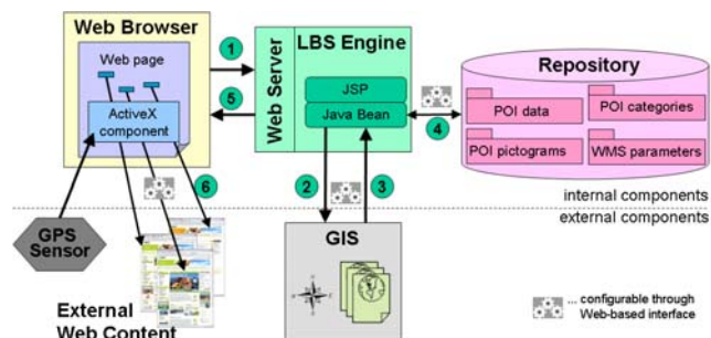
Fig 3. Architecture
