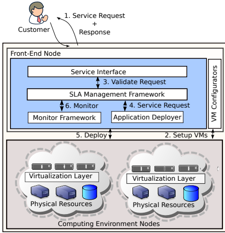
Fig. 1. CASViD Architecture.
